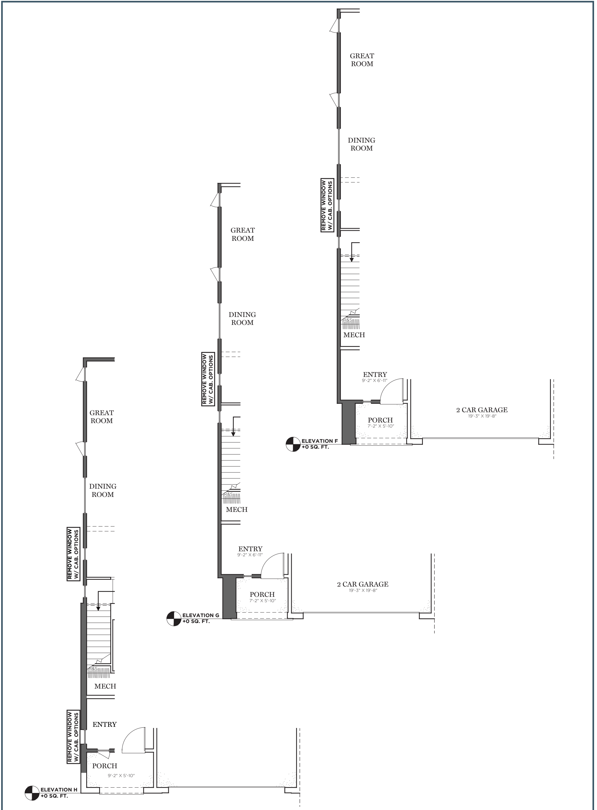
FIRST FLOOR MODIFY FLOOR PLAN OA DIMENSION 30 X 61
