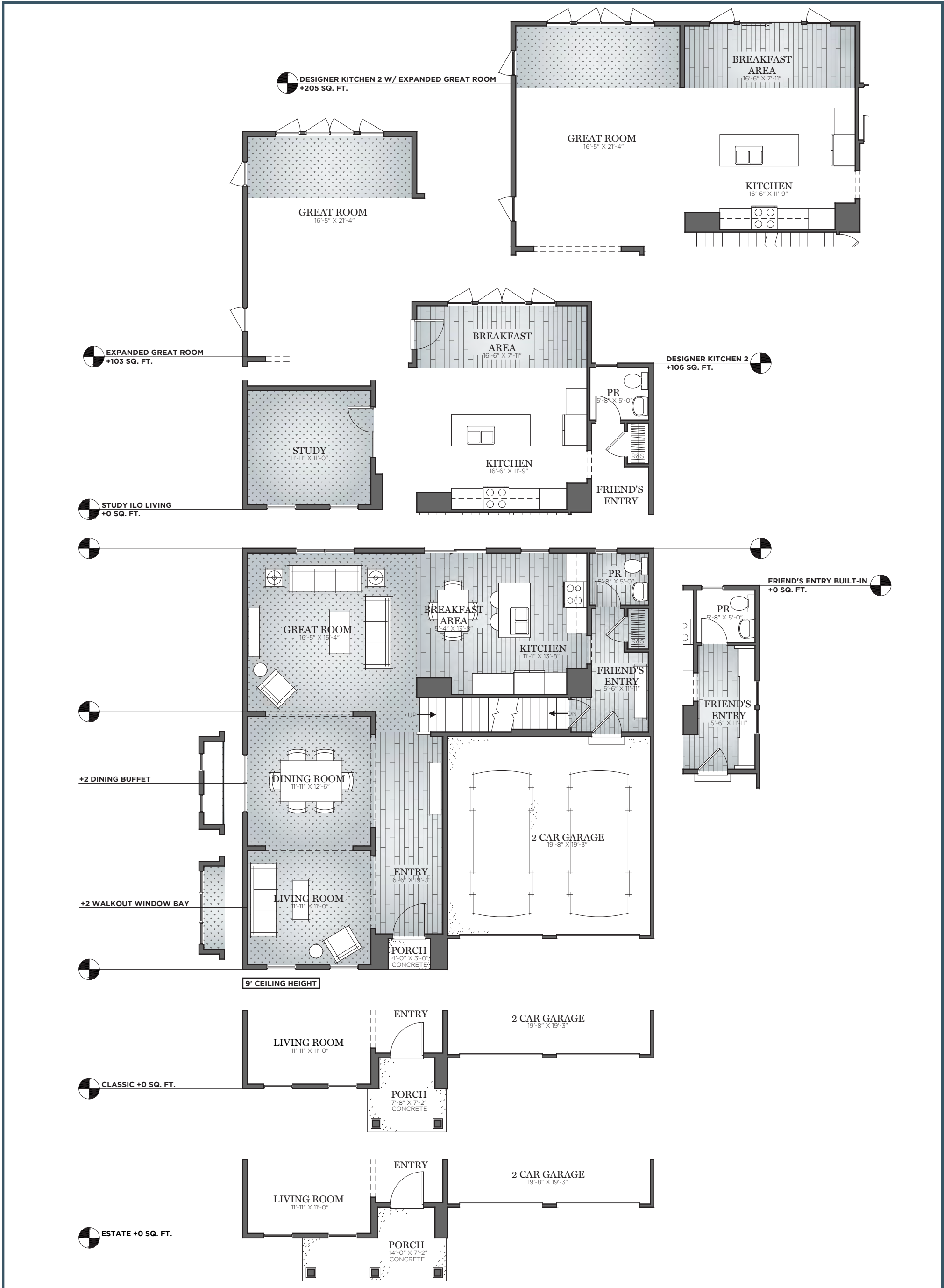
FIRST FLOOR MODIFY FLOOR PLAN OA DIMENSION 40 X 41
