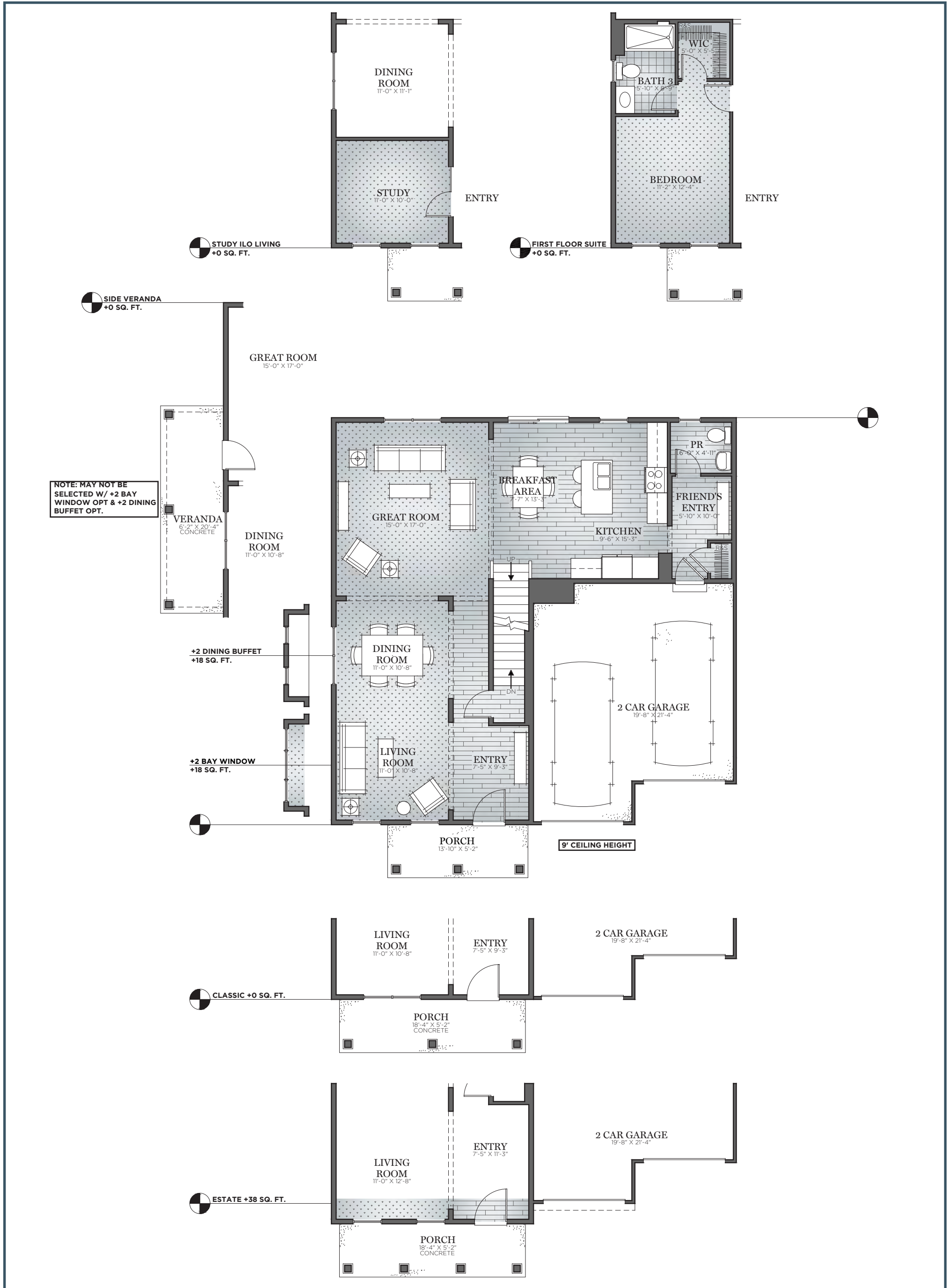
FIRST FLOOR MODIFY FLOOR PLAN OA DIMENSION 40 X 45
