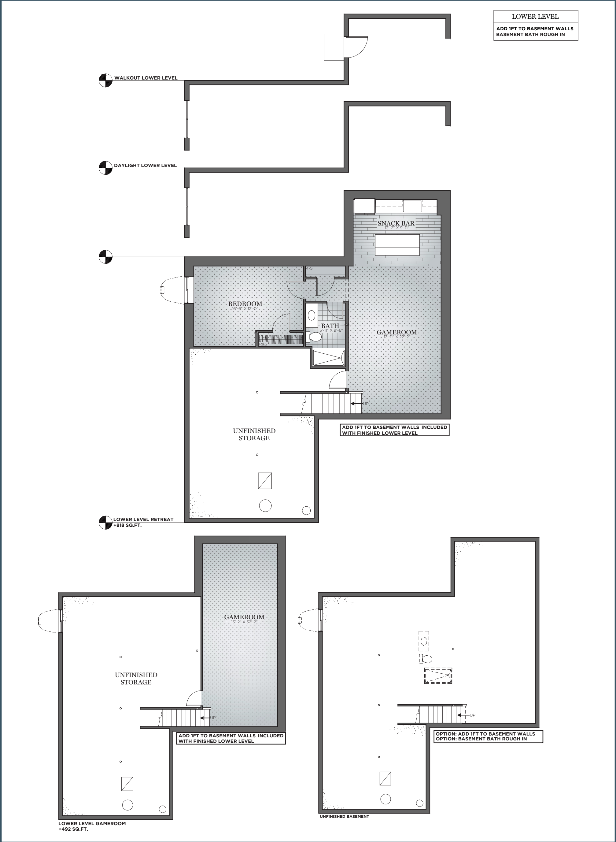
LOWER LEVEL MODIFY FLOOR PLAN OA DIMENSION 40 X 55
