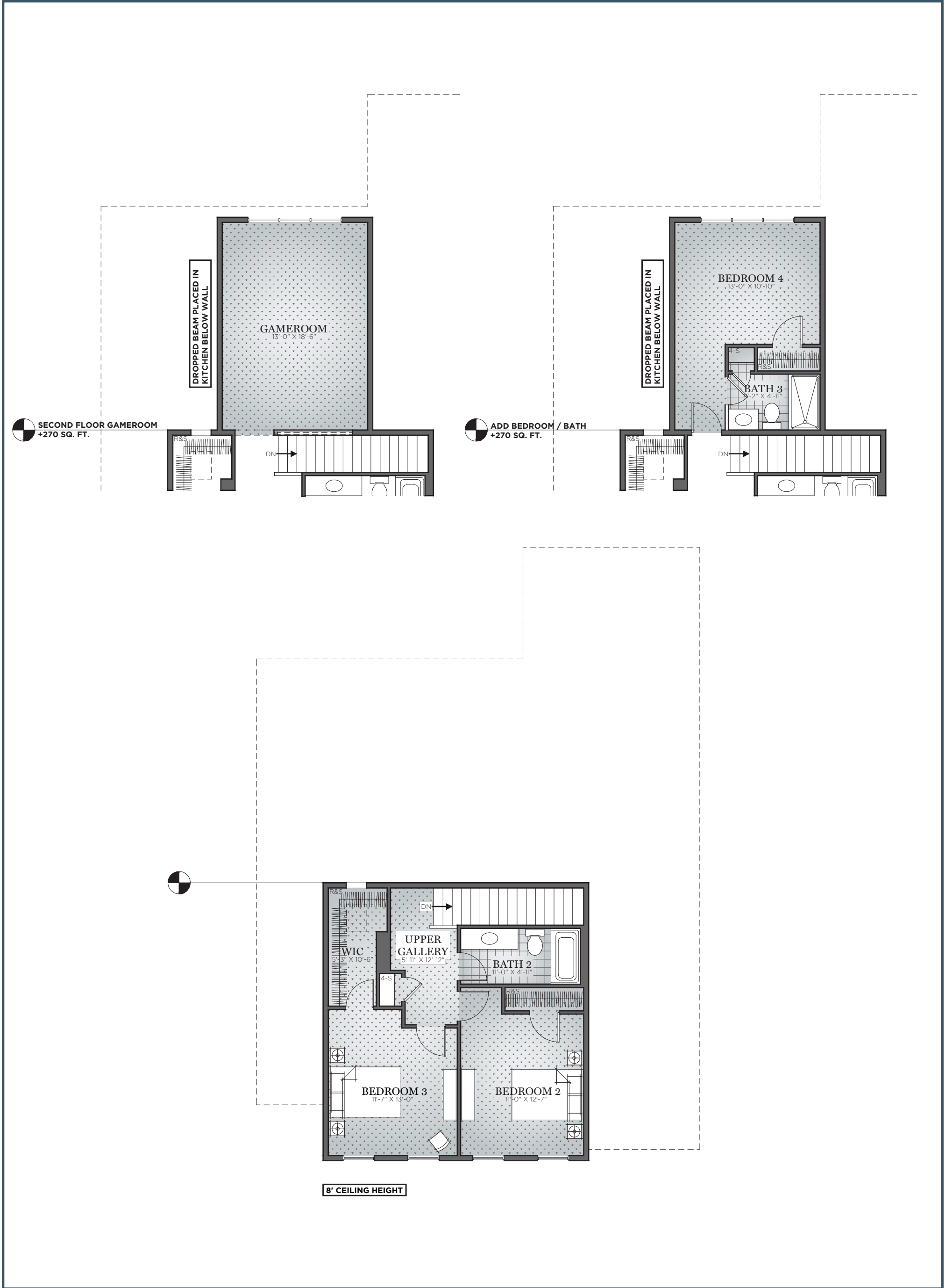
SECOND FLOOR MODIFY FLOOR PLAN OA DIMENSION 40 X 55
