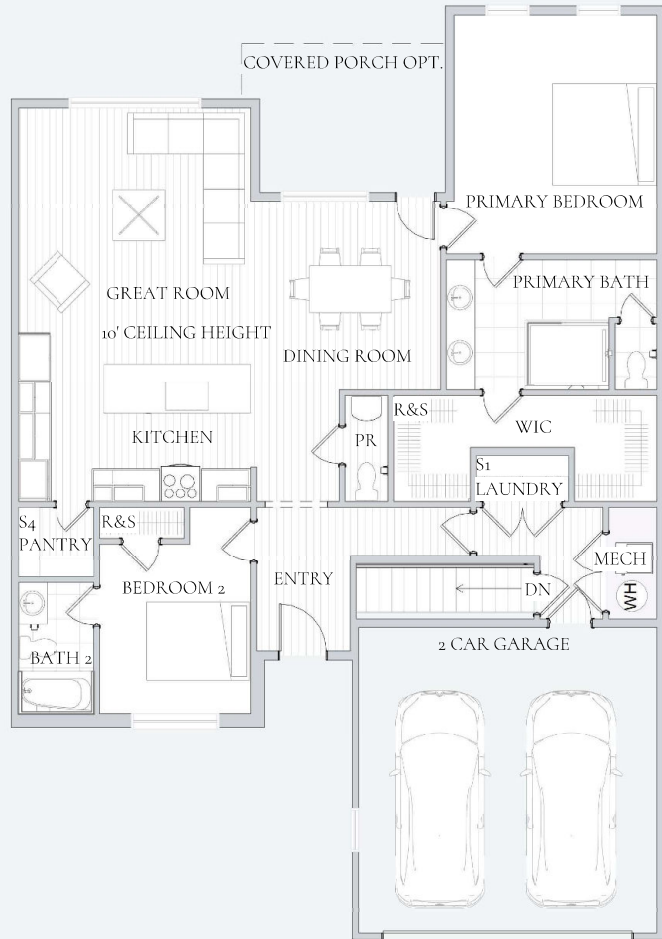
Elv. 10/15 1,554 sq. ft.
