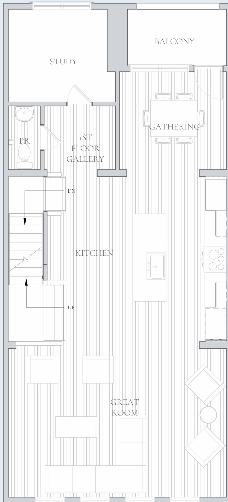
First Floor Ceiling Height 9' - 0"
