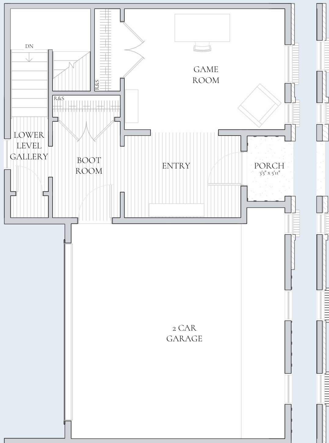
Lower Level Elevation 40.41.1 Ceiling Height 9'-0"
