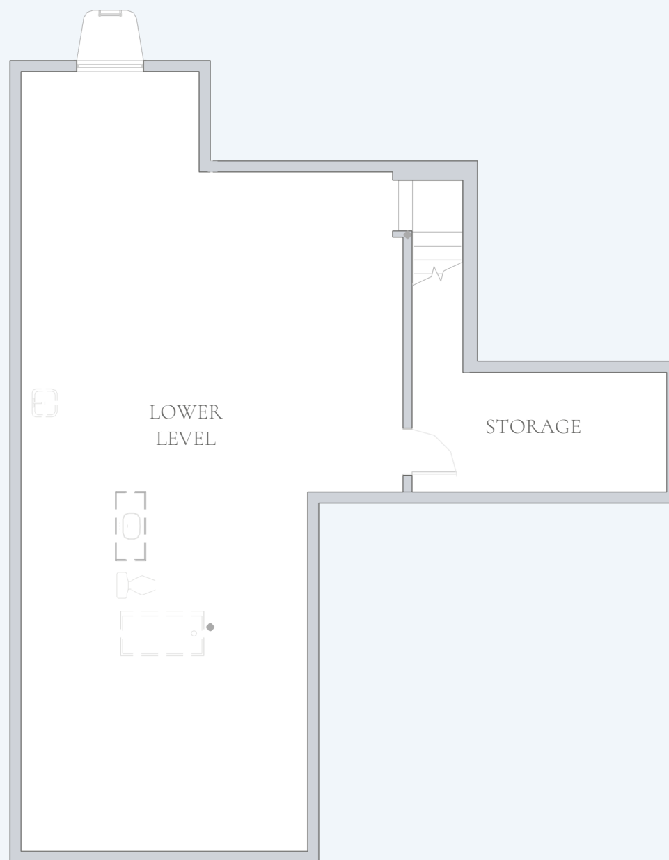
Lower Level Ceiling Height 8'-8" Option: Basement Bath Rough In Option: Basement Wet Bar Rough In
