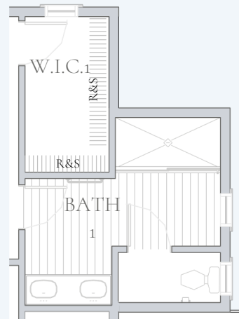
Bath 1 - Layout 6 +80 Sq. Ft.
