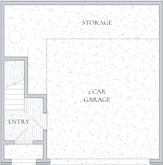
Lower Level 32.22.1 Ceiling Height 8'-0"
