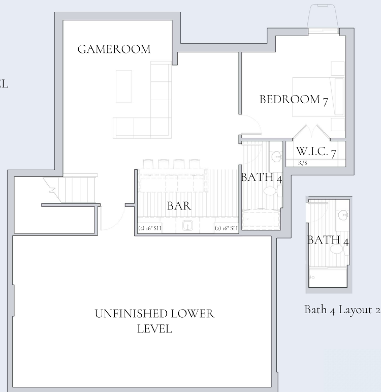
Lower Level Layout 3 w/ Bar ILO Unfinished Lower Level +843 Sq Ft.
