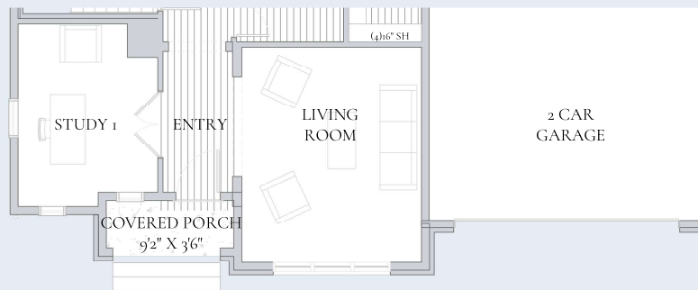
Elevation 20 + 57 Sqft
