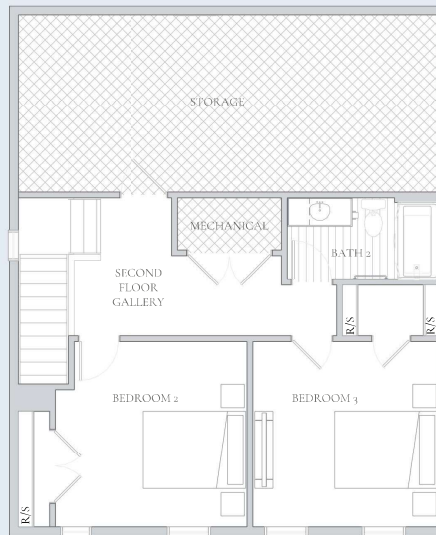
SECOND FLOOR PLAN EL. 60.12.1E CEILING HEIGHT 8'
