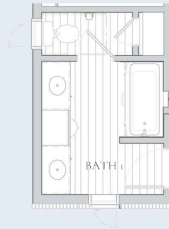
EL.10, 20, 30 BATH 1 LAYOUT4
