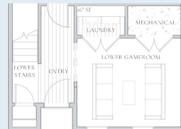
LOWER LEVEL PLAN EL. 52.11.2 THROUGH 52.32.1C LOWER LEVEL GAMEROOM ILO UNFINISHED +181 sq. ft.
