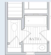
BATH 1 LAYOUT 4 EL. 52.11.2 THROUGH 52.32.1C
