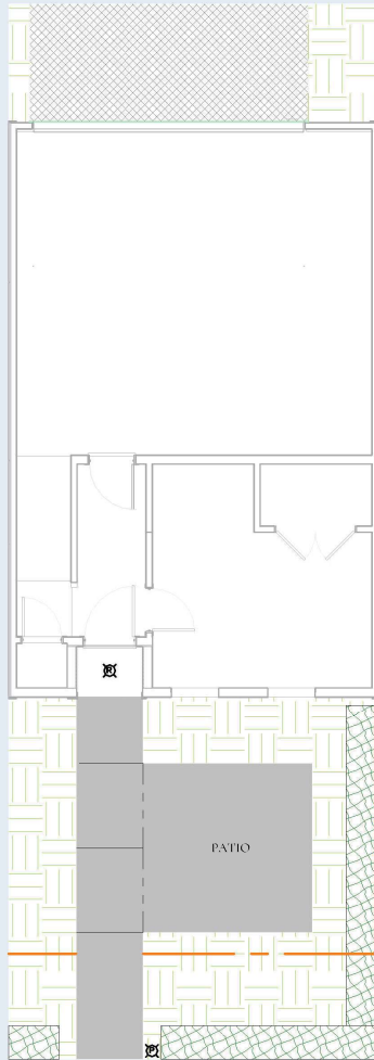
SITE PLAN INTERIOR
