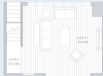
FIRST FLOOR PLAN EL. 52.11.3 & 52.11.1C +52 sq. ft.
