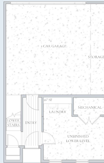
LOWER LEVEL PLAN CEILING HEIGHT 8'
